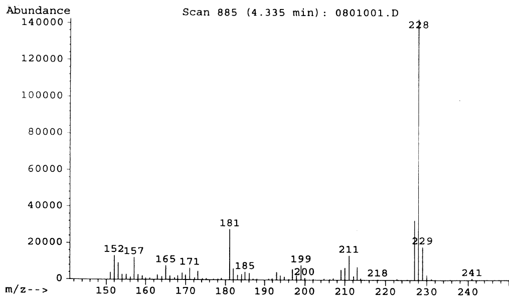
Fig. 3. Total-ion scan of peak A hydrolysed by \beta -glucosidase (see Experimental) for 12 h and subjected to direct-injection GC-MS (Ref. [19]). The molecular cluster at mass 229 [ M^+ ], 228 [ M ] and 227 [ M^- ] typical of resveratrol and at the retention time characteristic of the cis -isomer (4.3 min) is clearly seen. An identical mass ion spectrum but at a retention time of 5.7 min (characteristic of trans -resveratrol) was obtained when the same procedure was carried out on peak B.
