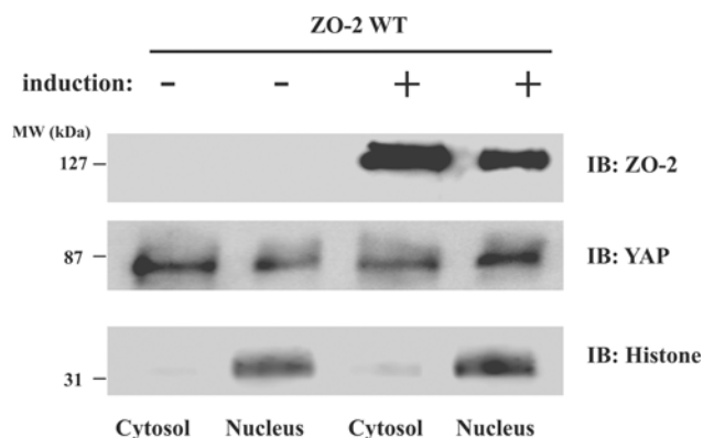
Figure S4 YAP2 accumulates in the nucleus in the presence of ZO-2-WT in HEK-293 cells
