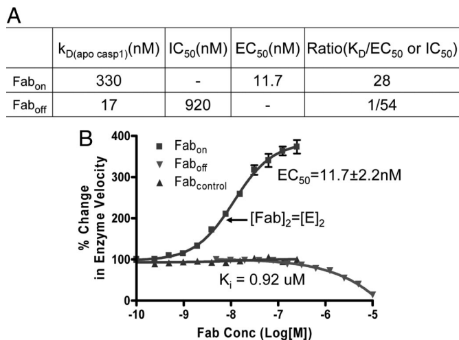
Fig. 4. Activation or inhibition of caspase-1 activity by Fabs. (A) Caspase-1 (5 nM) was preincubated with serial dilution of Fabs before assaying with fluorescent substrate Ac-WEHD-fmk at 100 \mu\text{M} concentration. The relative change in enzyme velocity was calculated by dividing the enzyme velocity at any given Fab concentration with the average velocity of enzyme in the absence of Fab. Nonlinear regression was used to fit the curve and calculate EC_{50} and K_i . (B) The ratios of K_D(\text{apo caspase-1}) for each Fab to the corresponding EC_{50} or IC_{50} were calculated from data in A and Fig. 3A.
