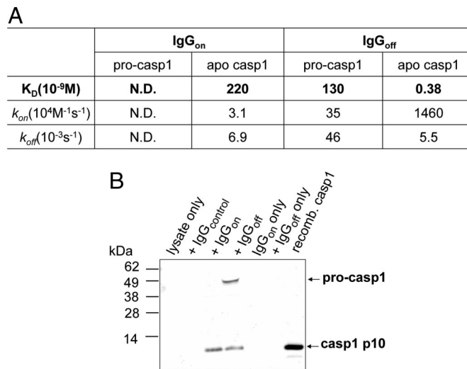
Fig. 5. IgG off binds to procaspase-1. (A) SPR analysis of IgGs by BIAcore. Kinetic analysis was performed by immobilizing procaspase-1 or apo caspase-1 on the CM5 chip and injecting serial dilutions of IgGs. BIAevaluation software was used to fit the recorded sensograms and determine the kinetic parameters. (B) Immunoprecipitation of procaspase-1 and apo caspase-1 from THP-1 lysates by IgGs. Monoclonal anti-caspase-1-p10 antibody (Calbiochem) that recognizes both procaspase-1 and caspase-1 p10 subunit was used in Western blot analysis.
