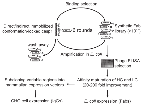
Fig. 2. Selection for conformation-selective antibodies. Six rounds of phage selection were performed for each target. Colonies were picked and tested by spot phage ELISA. Positive clones that showed both good affinity and selectivity were analyzed by DNA sequencing. HC and LC optimization were carried out for affinity maturation. Fabs and IgGs were expressed and purified in E. coli and mammalian cells, respectively. See Materials and Methods for details.
