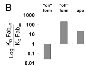
Fig. 3. Fabs are conformation-selective. (A) SPR analysis of Fabs by BIAcore. Kinetic analysis was performed by immobilizing different forms of caspase-1 on the CM5 chip and injecting serial dilutions of Fabs. BIAevaluation software was used to fit the recorded sensograms and determine the kinetic parameters. (B) The relative difference in K_D of Fabs binding to different forms of caspase-1 was calculated from data in A.
